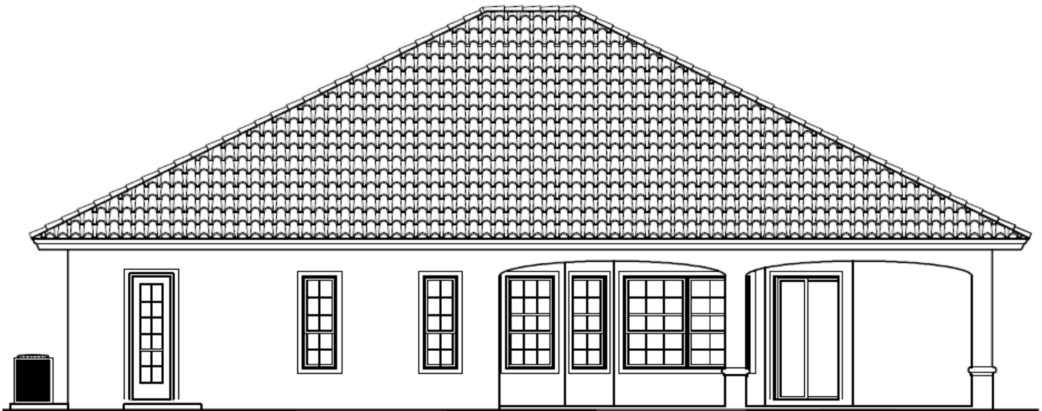
Rear Elevation
